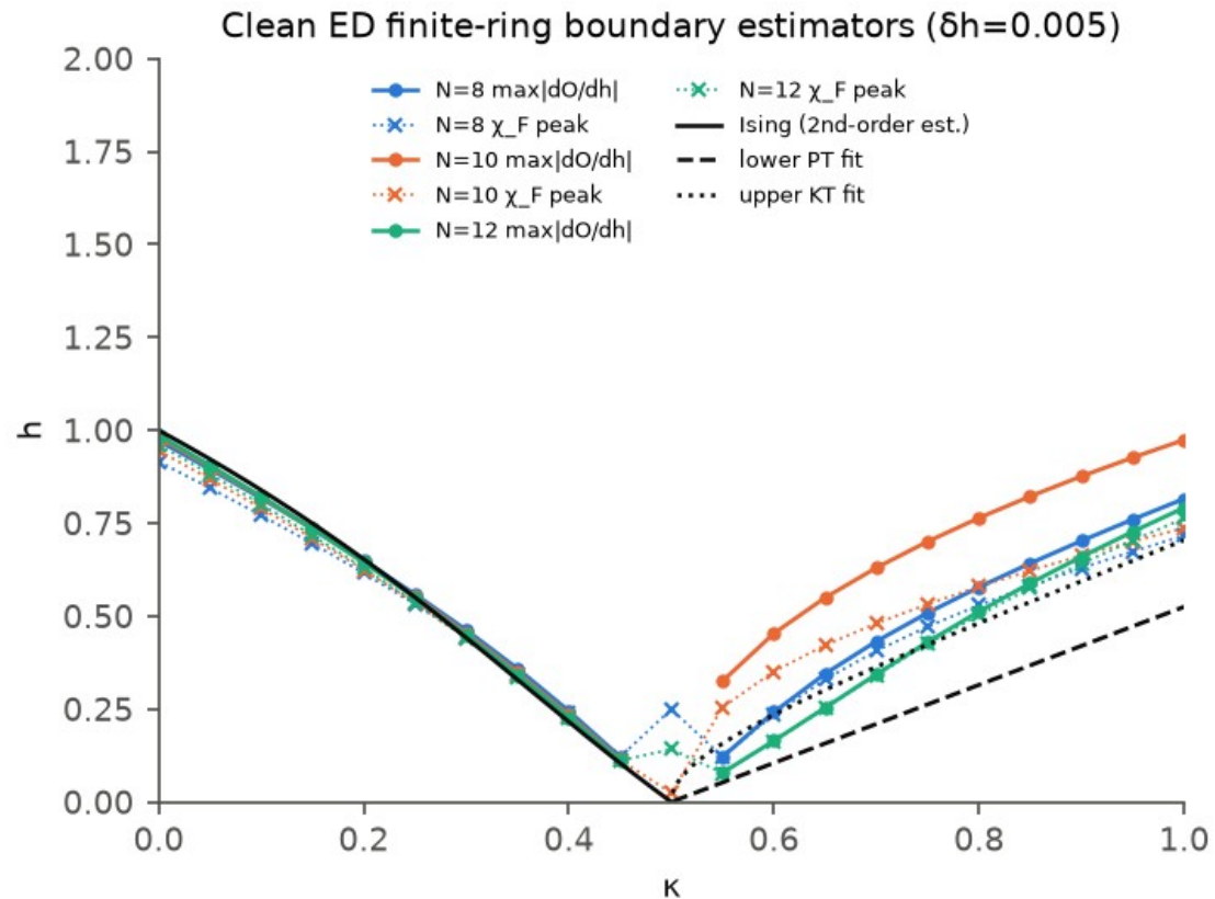
Boundary estimators from exact diagonalisation at N = 8, 10, 12 with the Ising, PT and KT reference curves.
